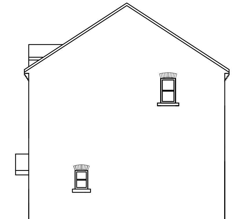
SIDE ELEVATION AS PROPOSED (1:100)
