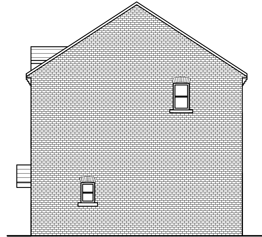
SIDE ELEVATION AS EXISTING (1:100)
