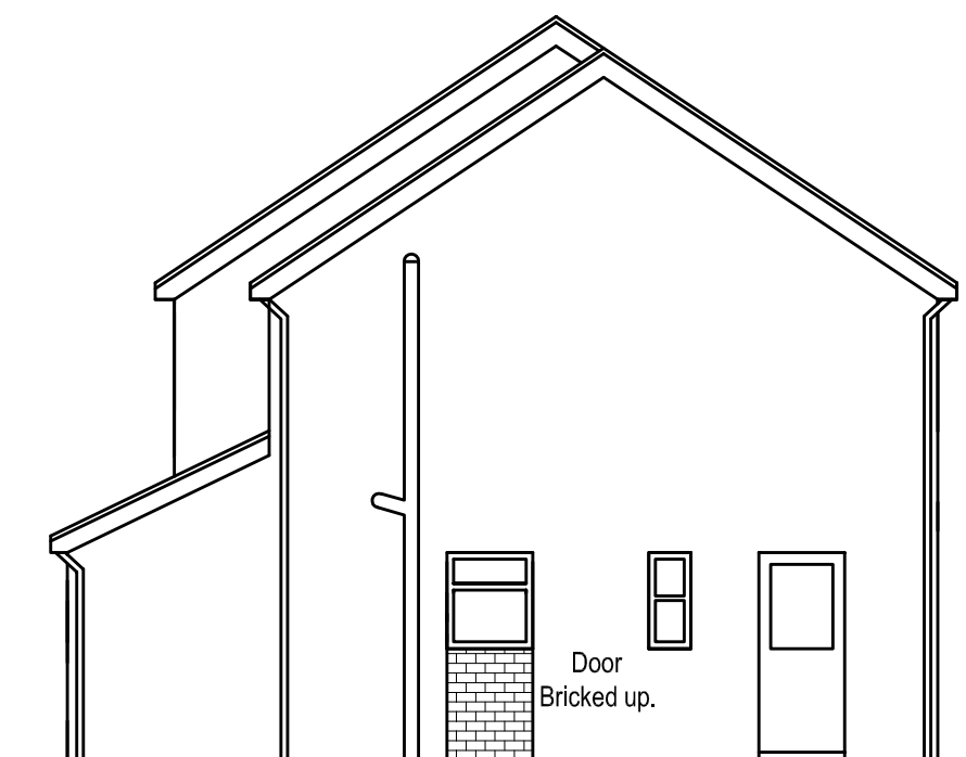
SIDE ELEVATION AS PROPOSED (1:100)
