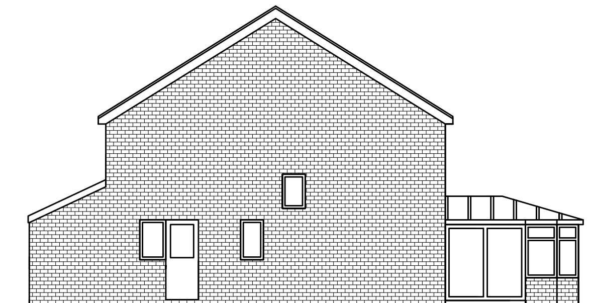
SIDE ELEVATION AS EXISTING (1:100)
