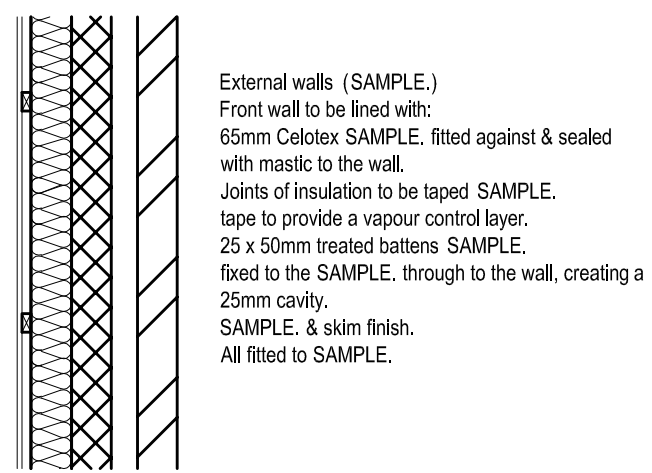
INSULATION UPGRADE TO WALLS DETAIL (NTS)
