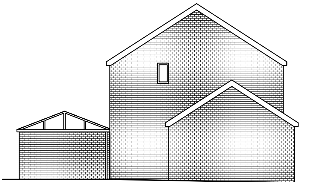
SIDE ELEVATION AS EXISTING (1:100)
