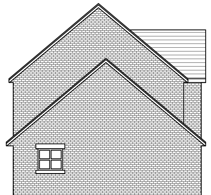
SIDE ELEVATION AS PROPOSED (1:100)
